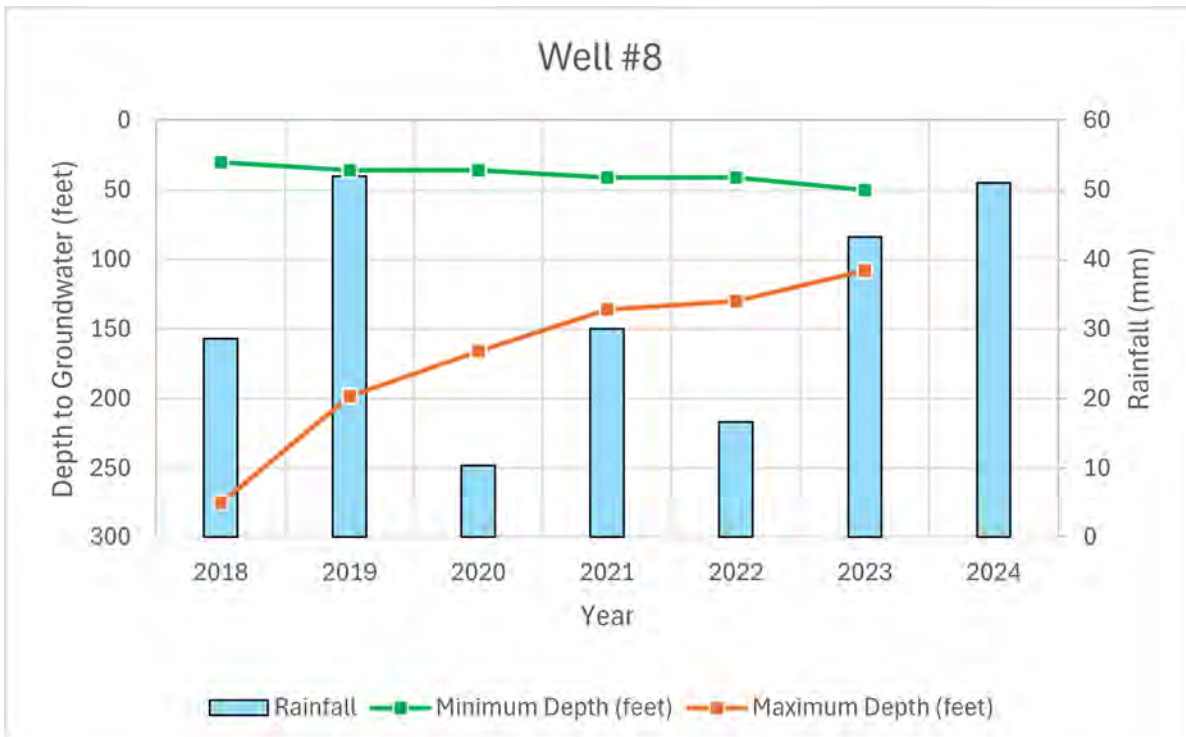
Figure 7 Well #8 levels.
