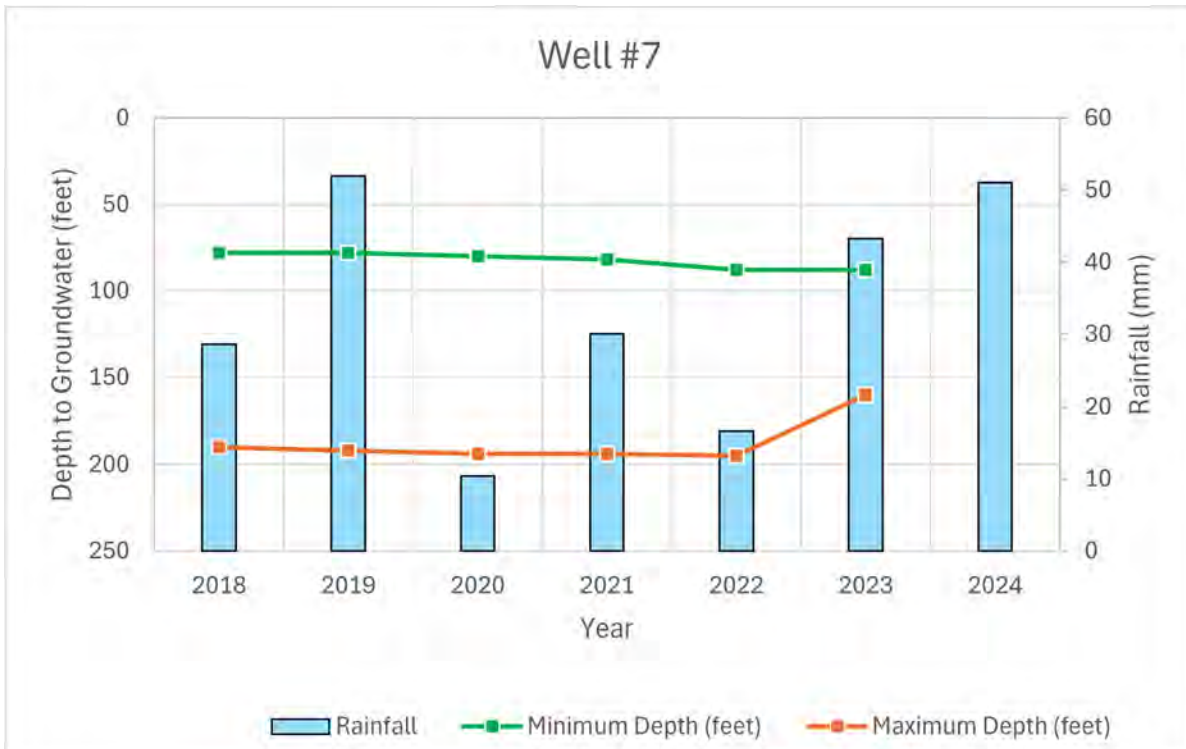
Figure 6 Well #7 levels.
