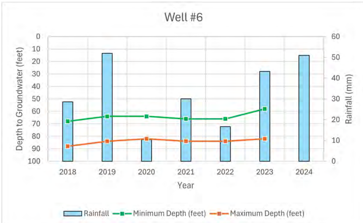
Figure 8 Well #6 levels.
