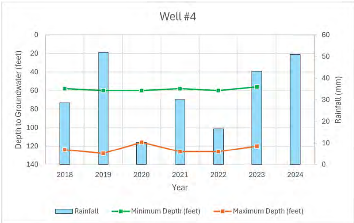
Figure 5 Well #4 levels.
